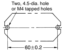
Mounting Holes
